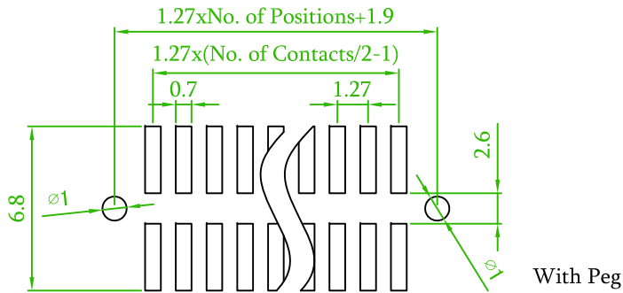
Recommended PCB Layout (PCB TOLERANCE ±0.1)
