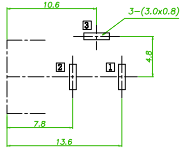
RECOMMENDED P.C.B. LAYOUT UNSPECIFIED TOLERANCE: \pm 0.05 (BOTTOM VIEW)
