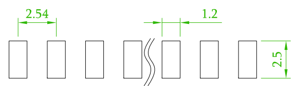
Recommended PCB Layout (PCB TOLERANCE ±0.1)
