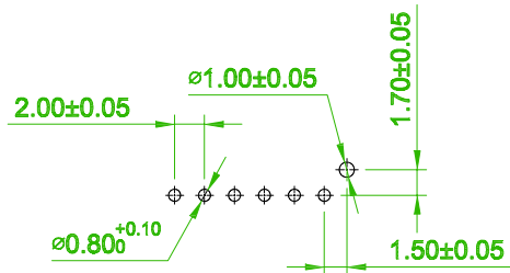
RECOMMENDED P.C. BOARD HOLE DIMM.
