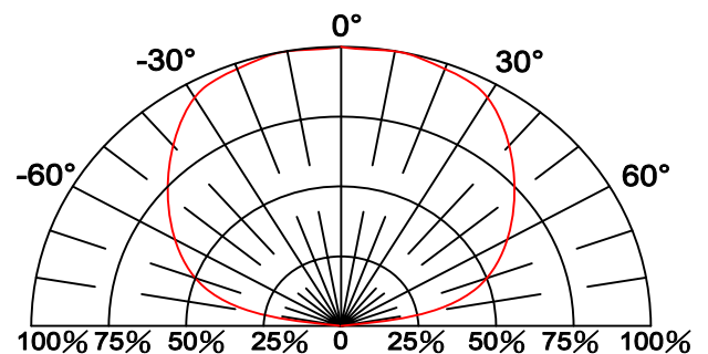
Fig.6 Directive Radiation
